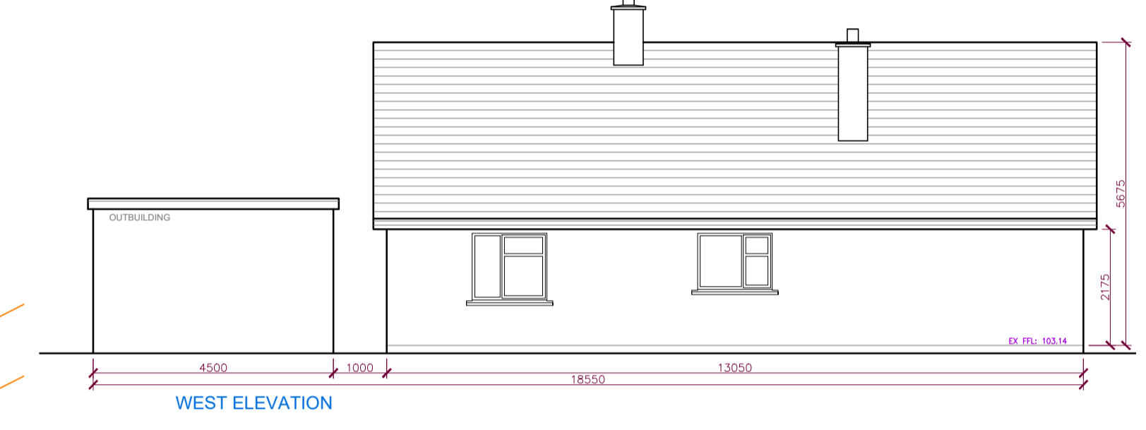
ELEVATIONS OF EXISTING DWELLING HOUSE & OUTBUILDINGS TO BE DEMOLISHED
