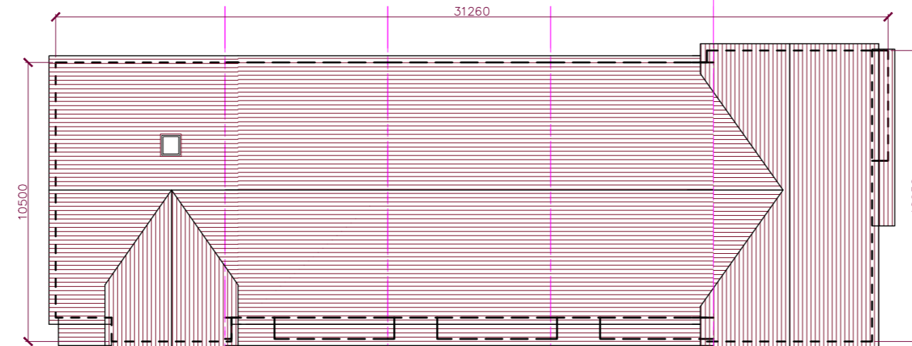
ROOF PLAN
