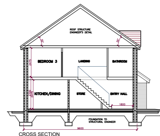
CROSS SECTION
