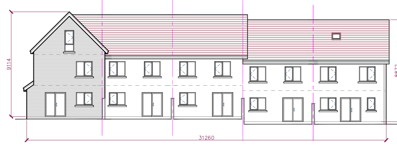
WEST ELEVATION
