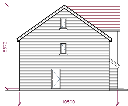
SOUTH ELEVATION
