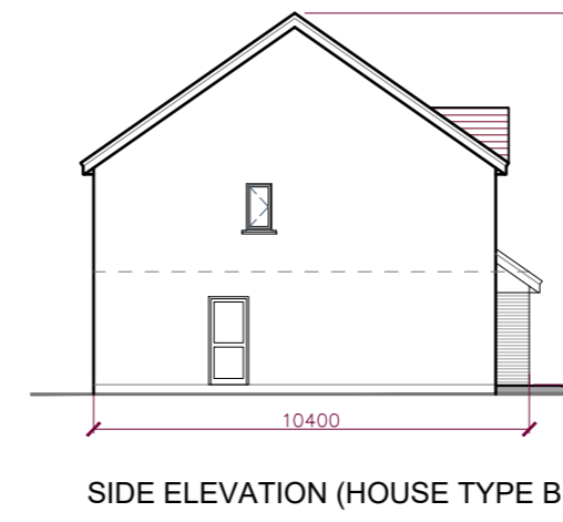
SIDE ELEVATION (HOUSE TYPE B)
