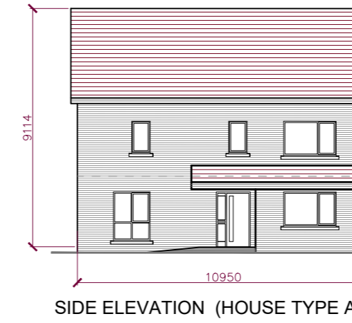
SIDE ELEVATION (HOUSE TYPE A)
