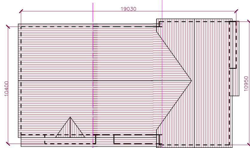
ROOF PLAN
