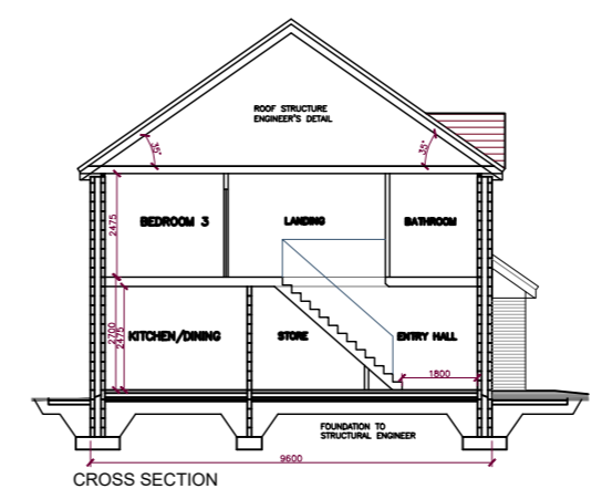
CROSS SECTION
