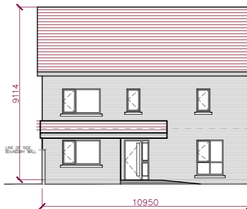
SIDE ELEVATION (HOUSE TYPE A)
