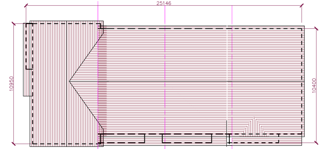
ROOF PLAN
