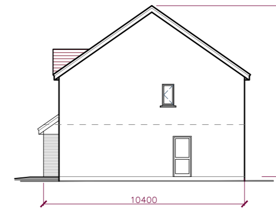
SIDE ELEVATION (HOUSE TYPE B)
