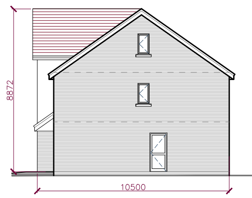
NORTH ELEVATION
