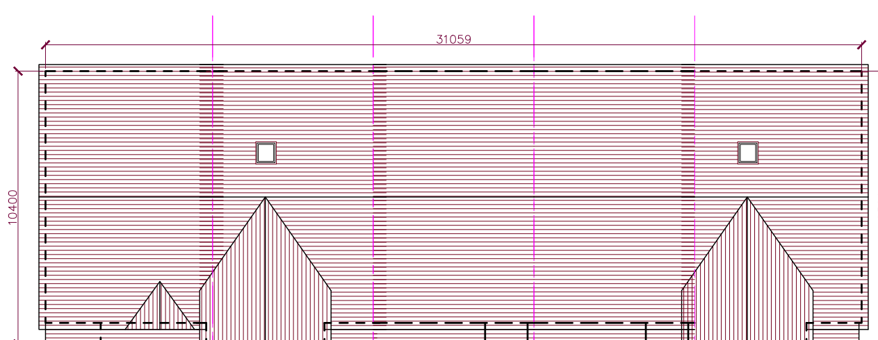
ROOF PLAN
