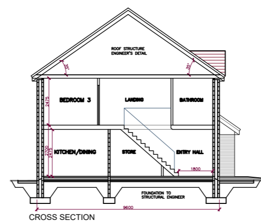
CROSS SECTION
